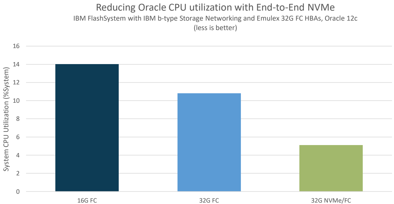
Figure 7. Oracle Server CPU Efficiency
