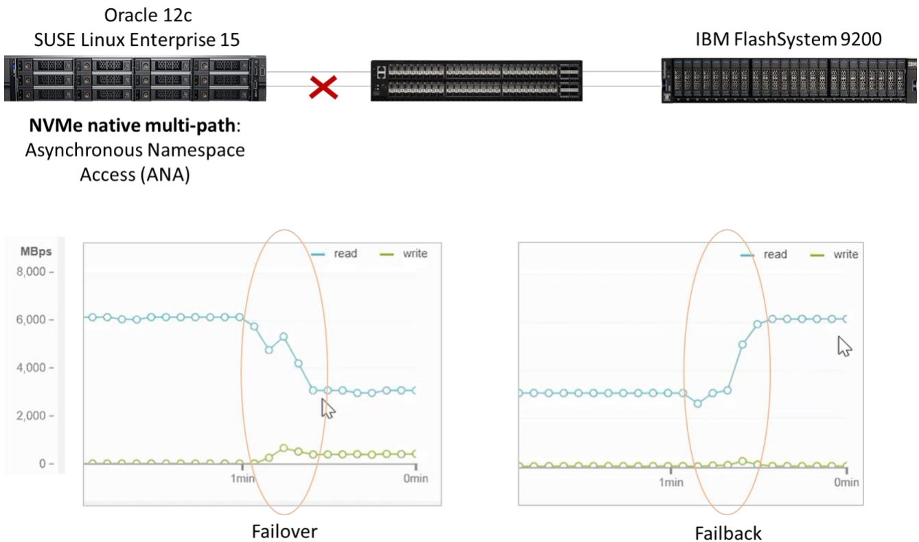
Figure 8. ANA Multipath Failover
