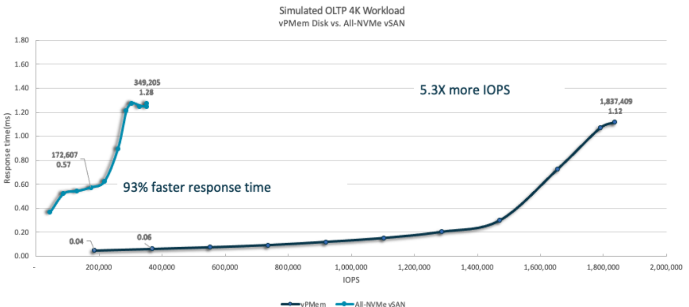
Figure 14. Simulated OLTP Workload: vPMem Disk versus All-NVMe vSAN
