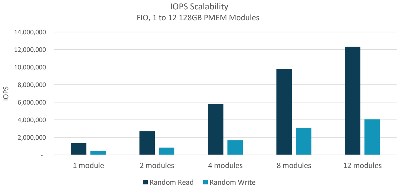
Figure 10. Near-linear IOPS Scalability
