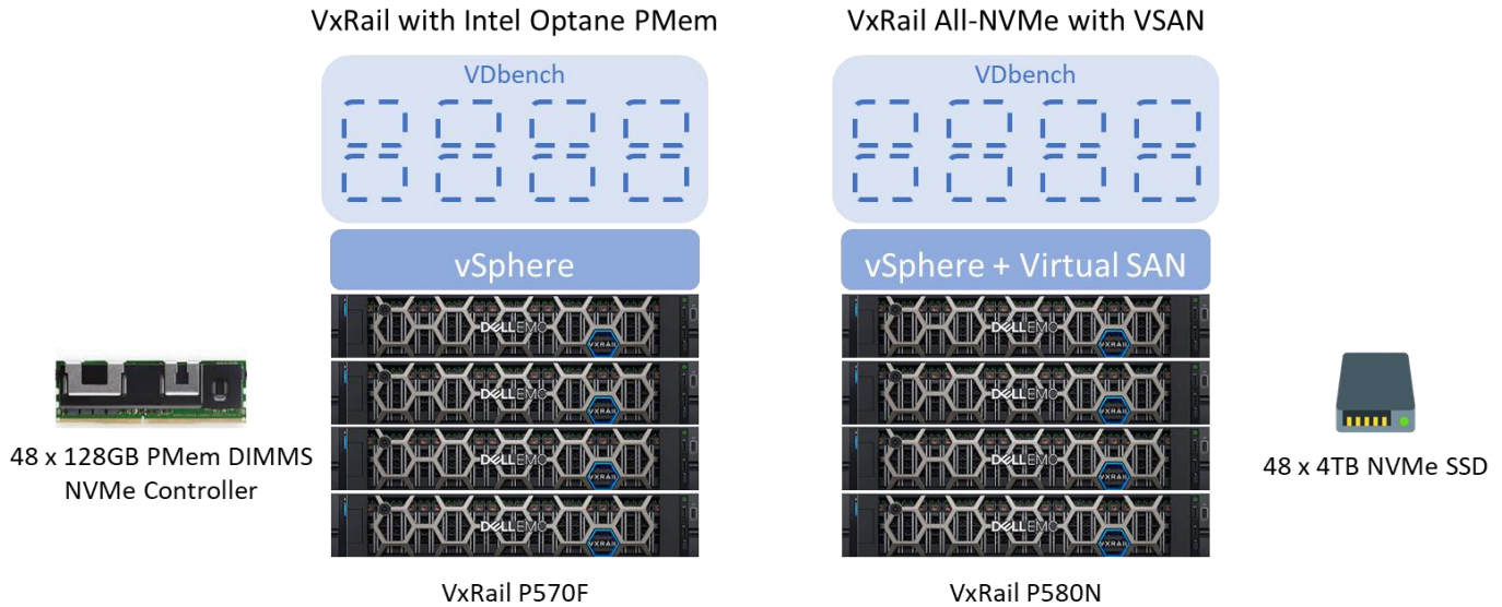
Figure 13. Simulated OLTP Workload Test Bed
