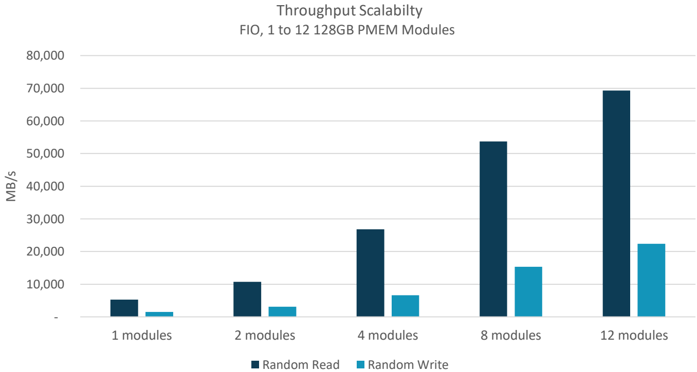
Figure 11. Near-linear Throughput Scalability
